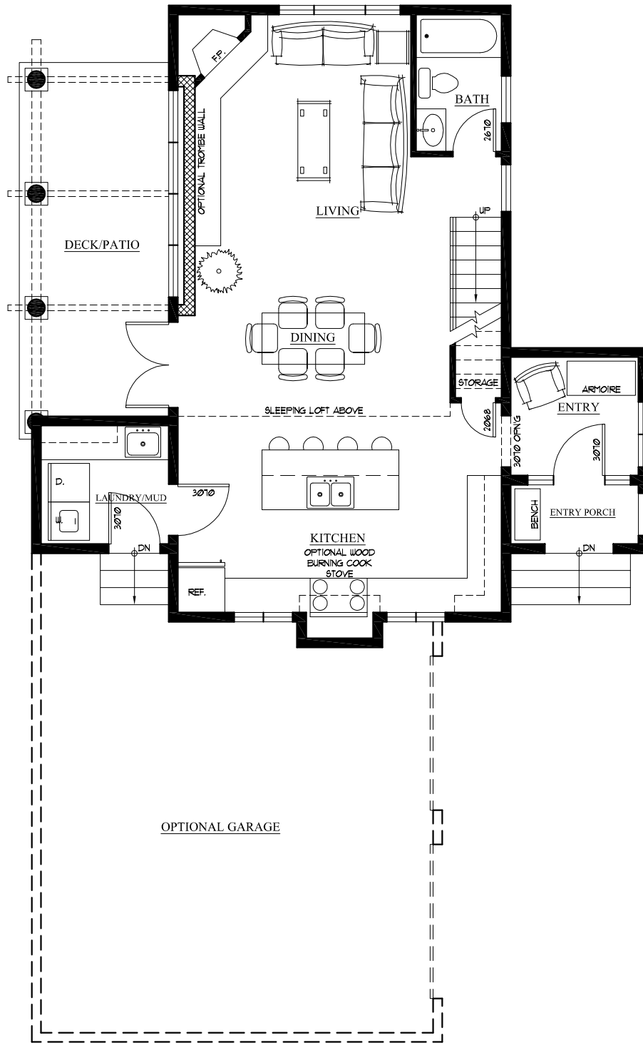
MAIN FLOOR PLAN 0 1 2 4 8 12 FT.
